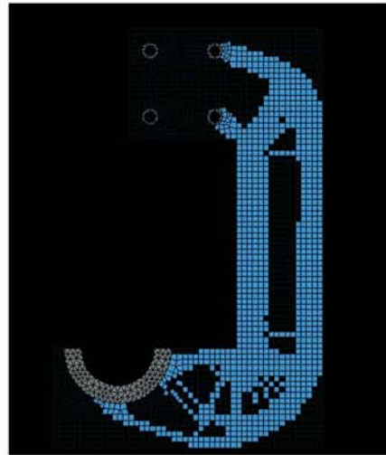
Topology optimization for Mechanical Design
