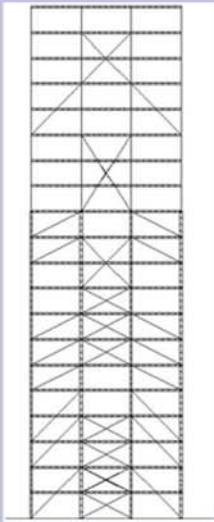
Form suggestion of multi-stories building from Topology optimization
